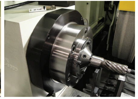
Custom spring-loaded autodriven
