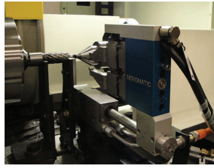
Automatic in-process sizing gage
