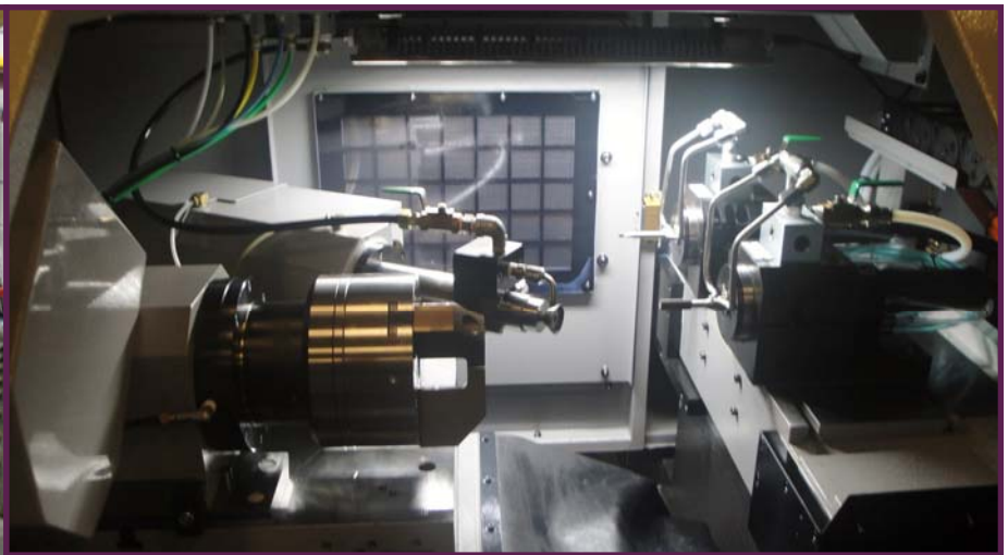
Electric rotary dresser and two (2) GMN 90,000 rpm spindles.
